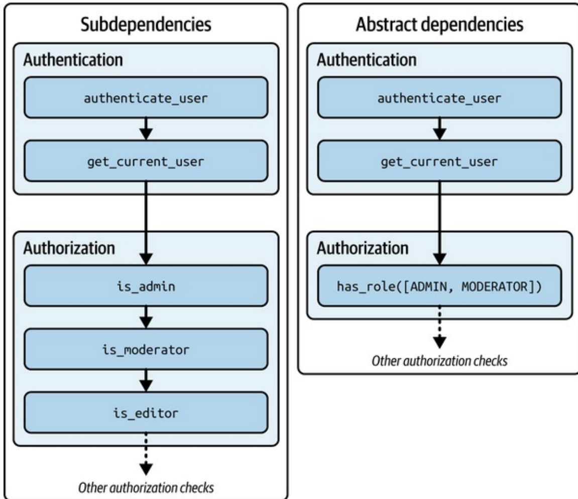
Figure 8-13. Approaches for implementing complex RBAC models
