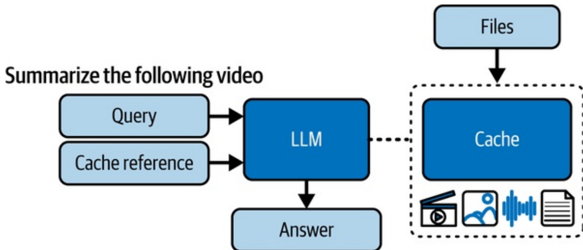
Figure 10-3. System architecture for context caching
