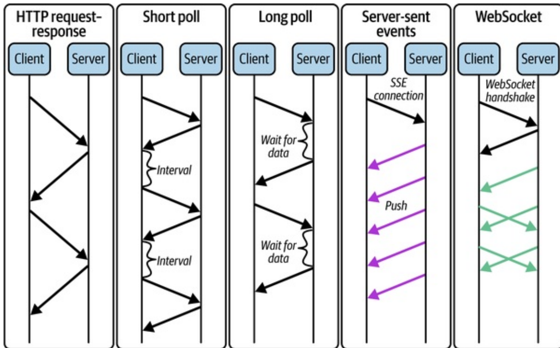
Figure 6-7. Comparison of web communication mechanisms
