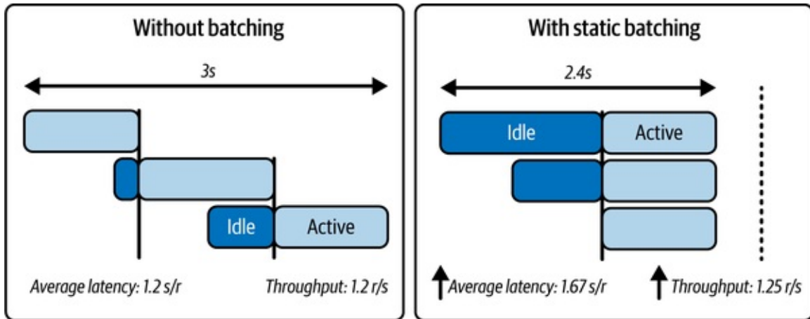
Figure 5-14. LLM server response latency and throughput with and without batching
