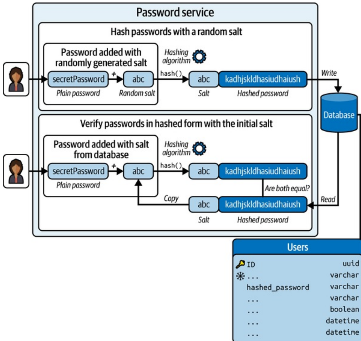
Figure 8-6. Password hash salting mechanism
