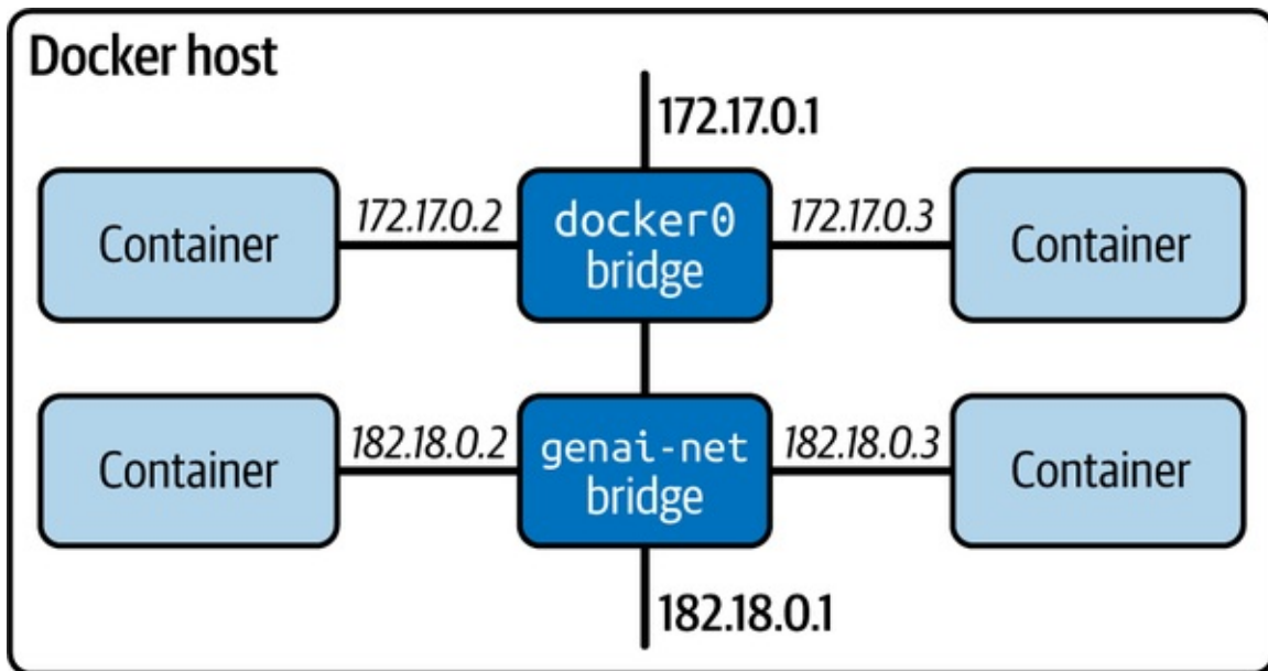
Figure 12-10. Isolated bridge networks
