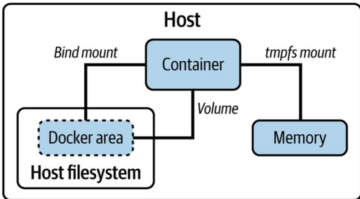
Figure 12-7. Docker storage mounts
