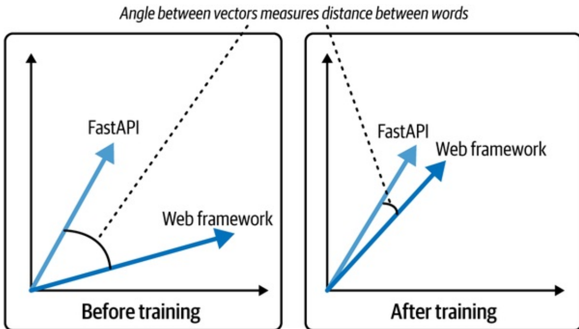
Figure 3-7. Training latent space of transformer network using embedding vectors
