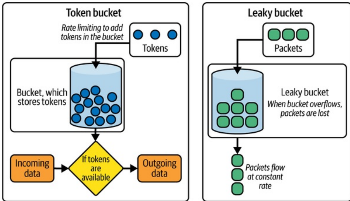
Figure 9-2. Comparison of rate-limiting strategies
