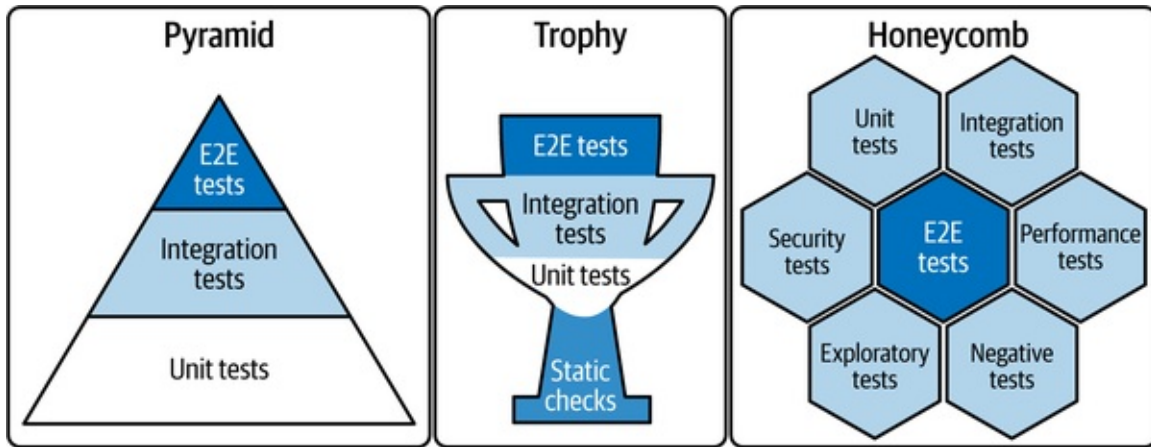
Figure 11-7. Visualization of testing strategies
