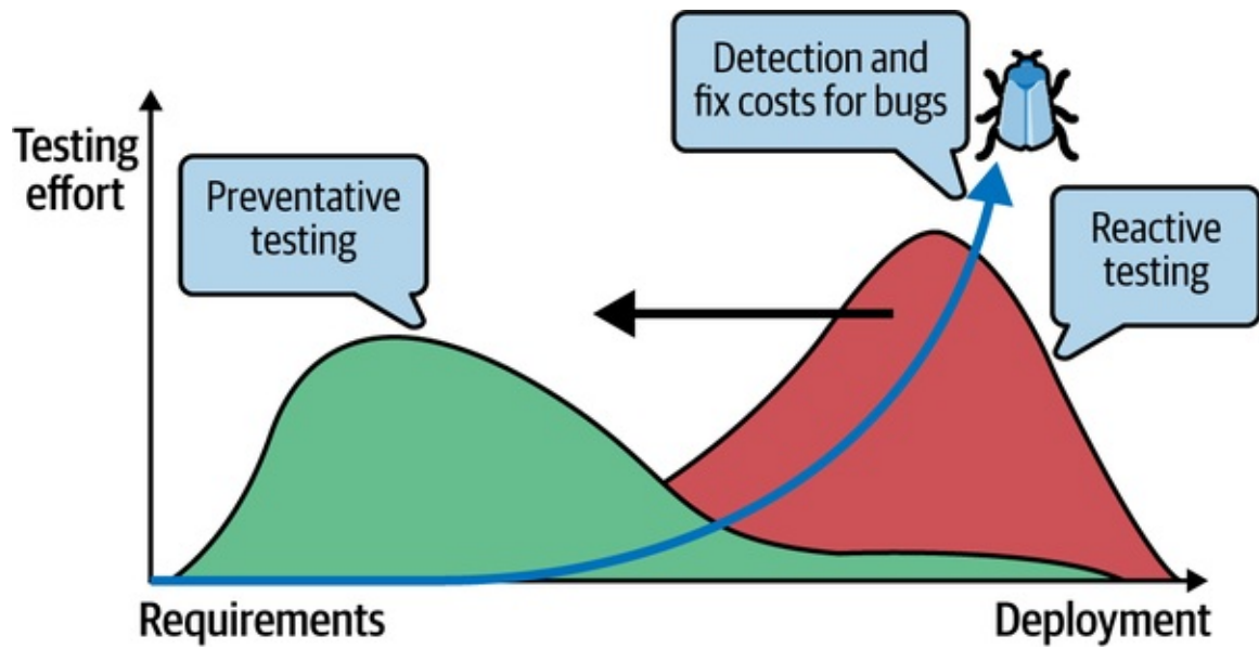
Figure 11-3. Shift-left software testing
