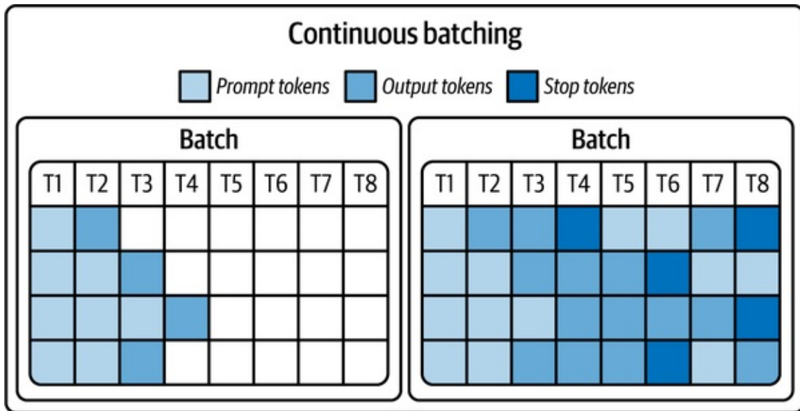
Figure 5-16. Dynamic/continuous batching with variable batch size
