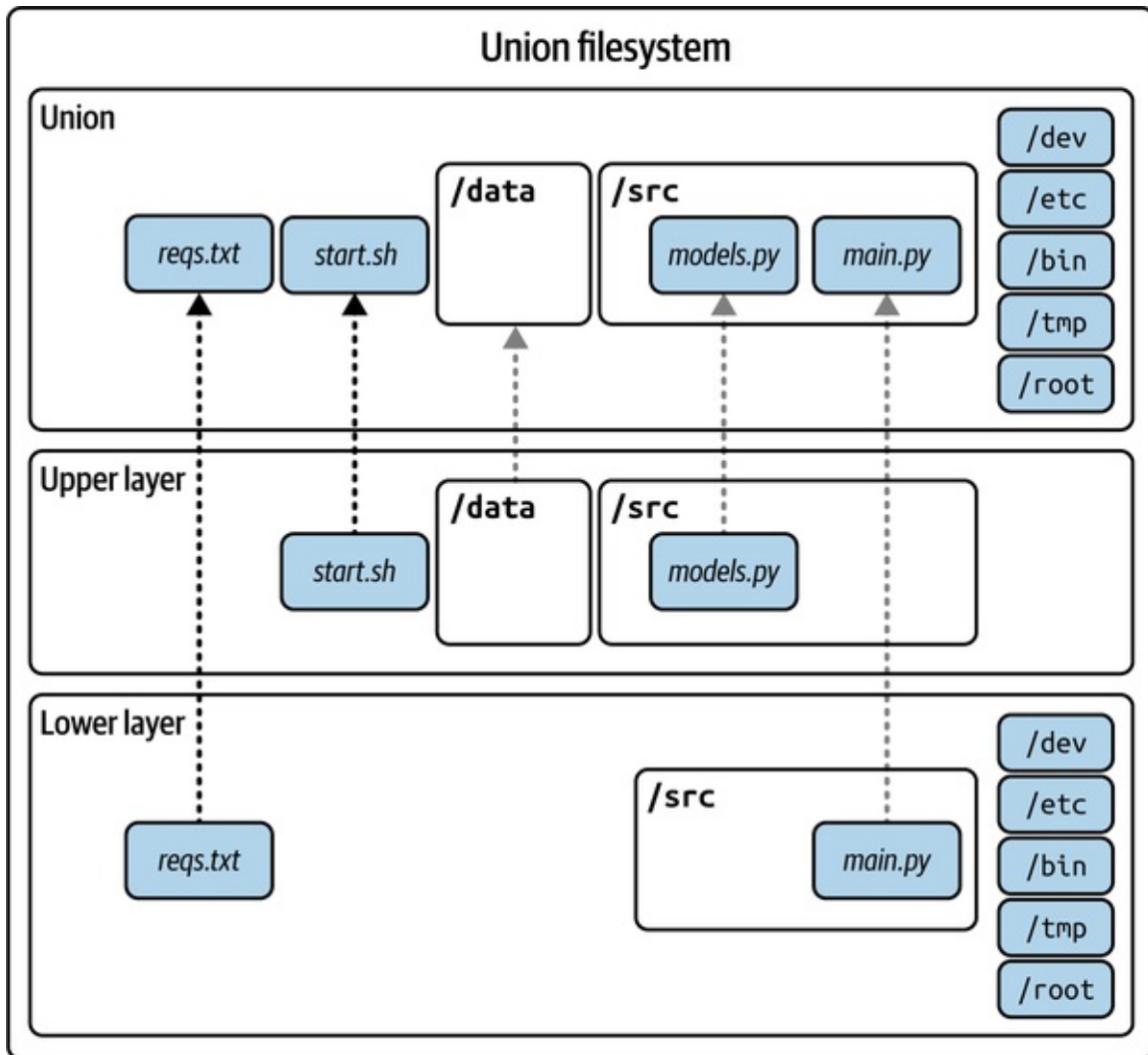
Figure 12-5. Unified virtual filesystem from multiple filesystems
