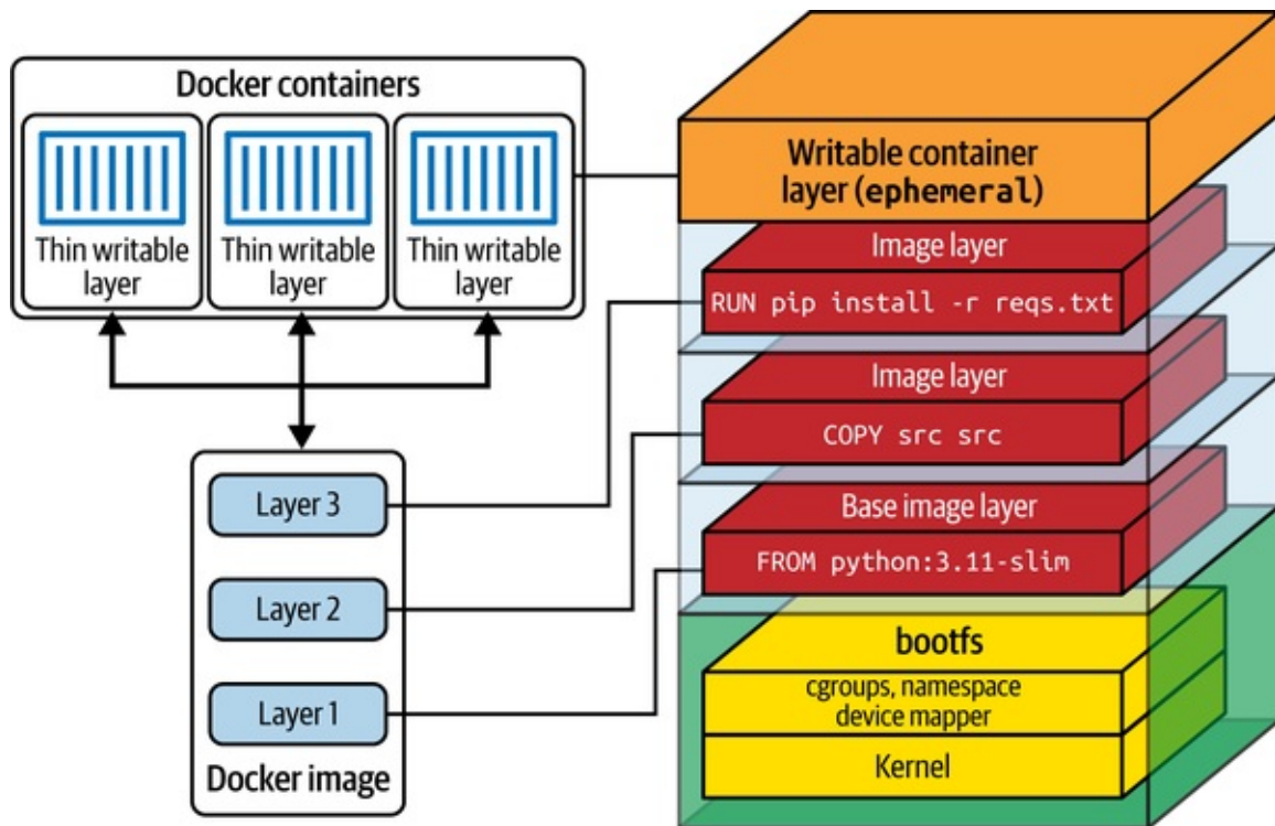
Figure 12-6. Layered Unionfs filesystem architecture
