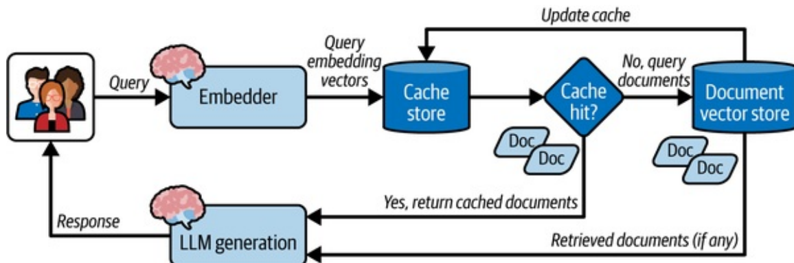
Figure 10-1. Semantic caching in RAG system architecture
