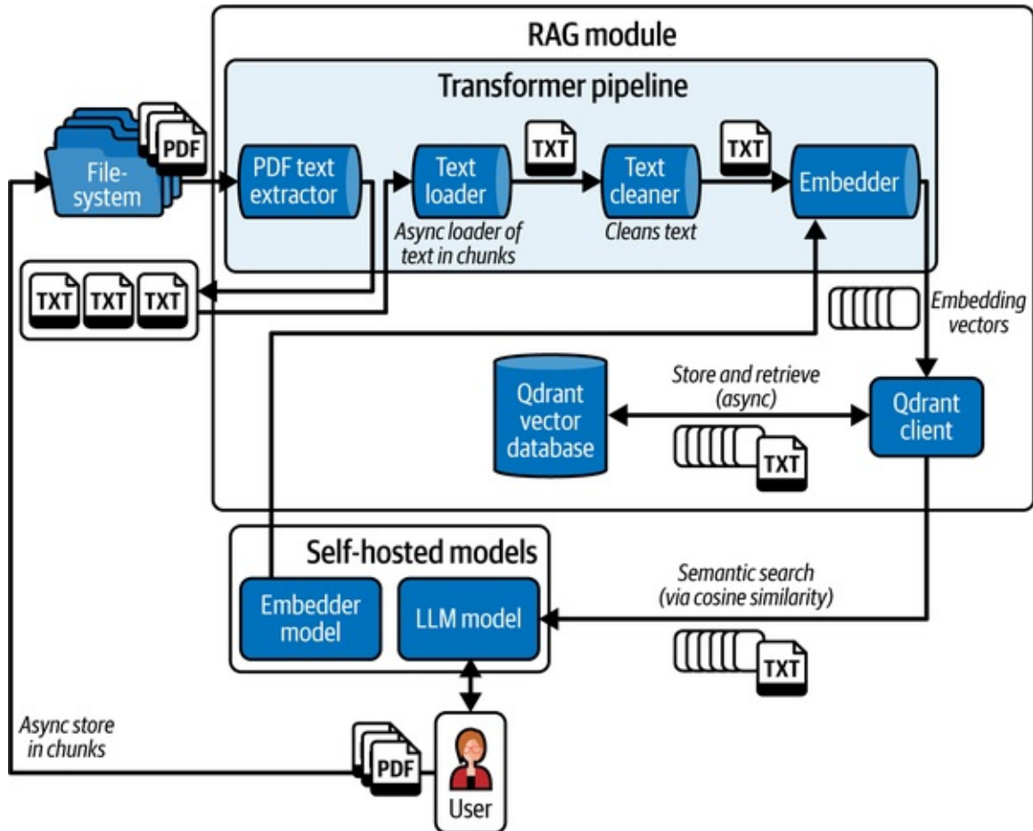
Figure 5-11. Detailed RAG data processing pipeline
