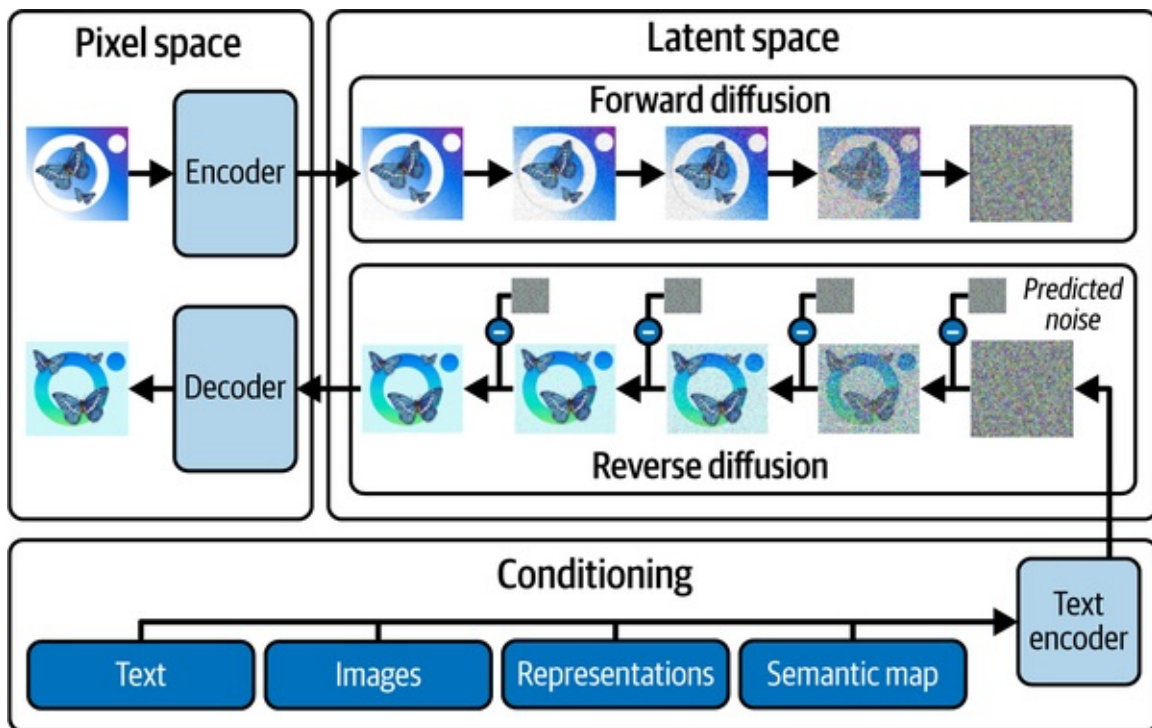
Figure 3-17. Stable Diffusion training and inference
