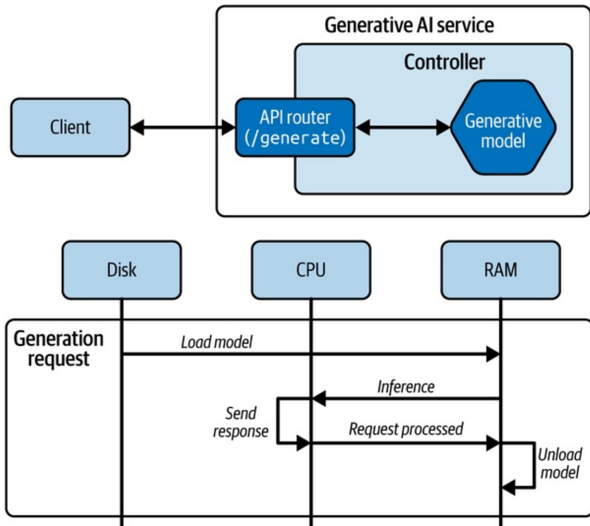
Figure 3-28. Loading and using models on every request
