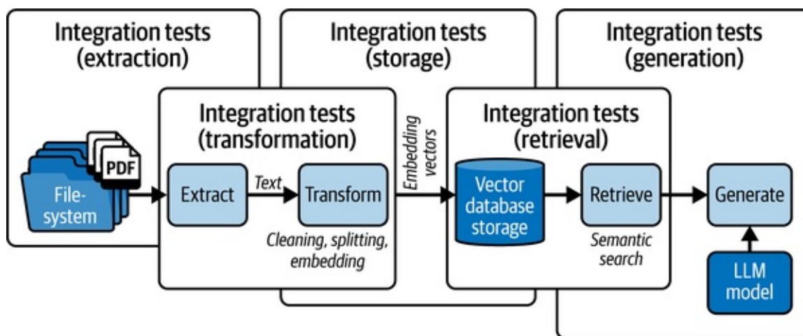
Figure 11-10. Integration test boundaries visualized on the RAG data pipeline diagram
