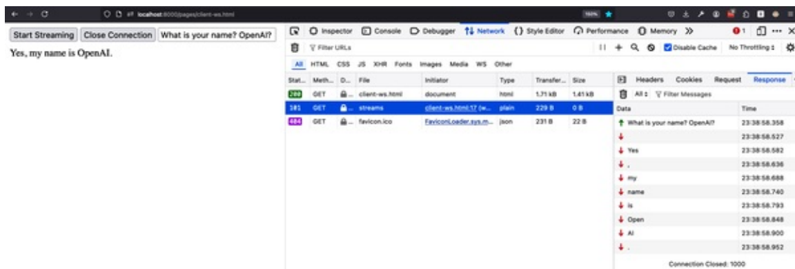
Figure 6-9. Incoming stream from the WebSocket endpoint
