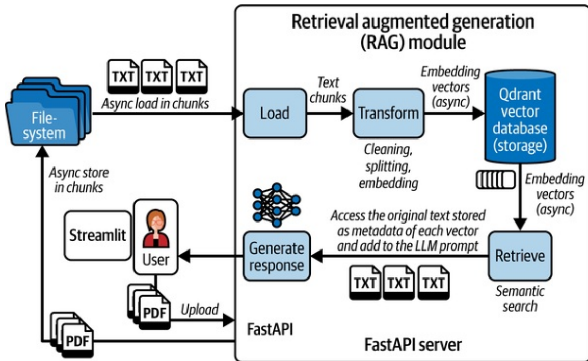
Figure 5-9. Talk to your documents system architecture
