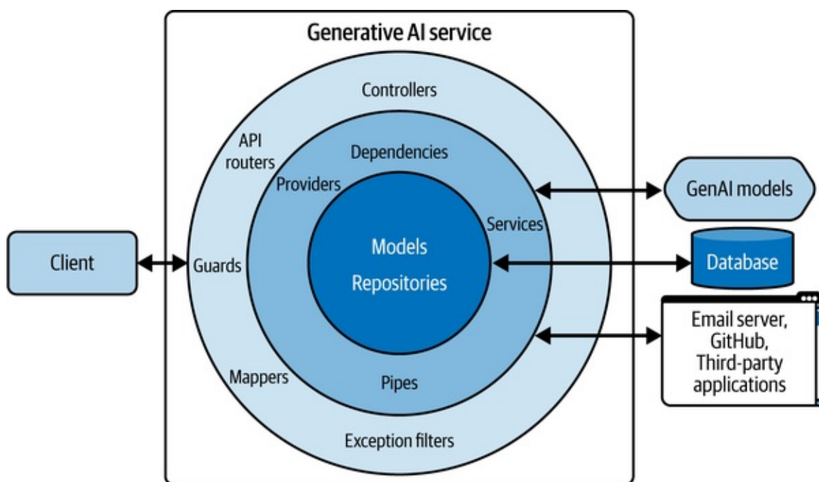
Figure 2-3. Onion design pattern
