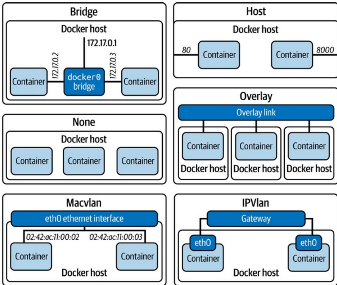
Figure 12-9. Docker networking drivers
