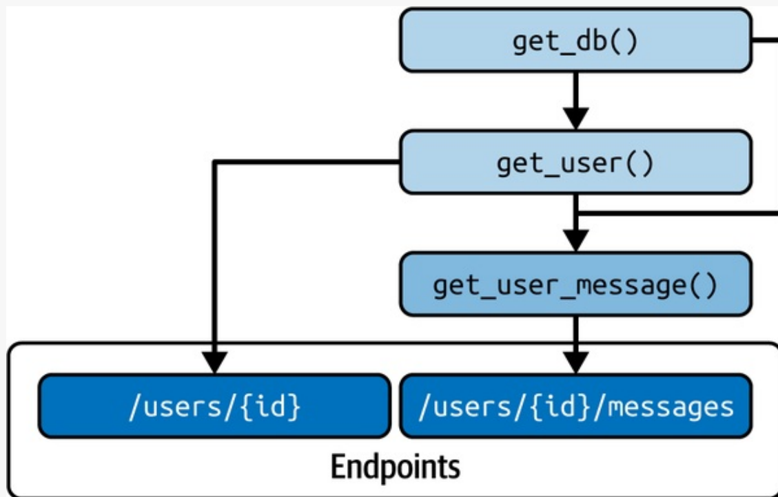
Figure 2-2. Dependency injection in FastAPI
