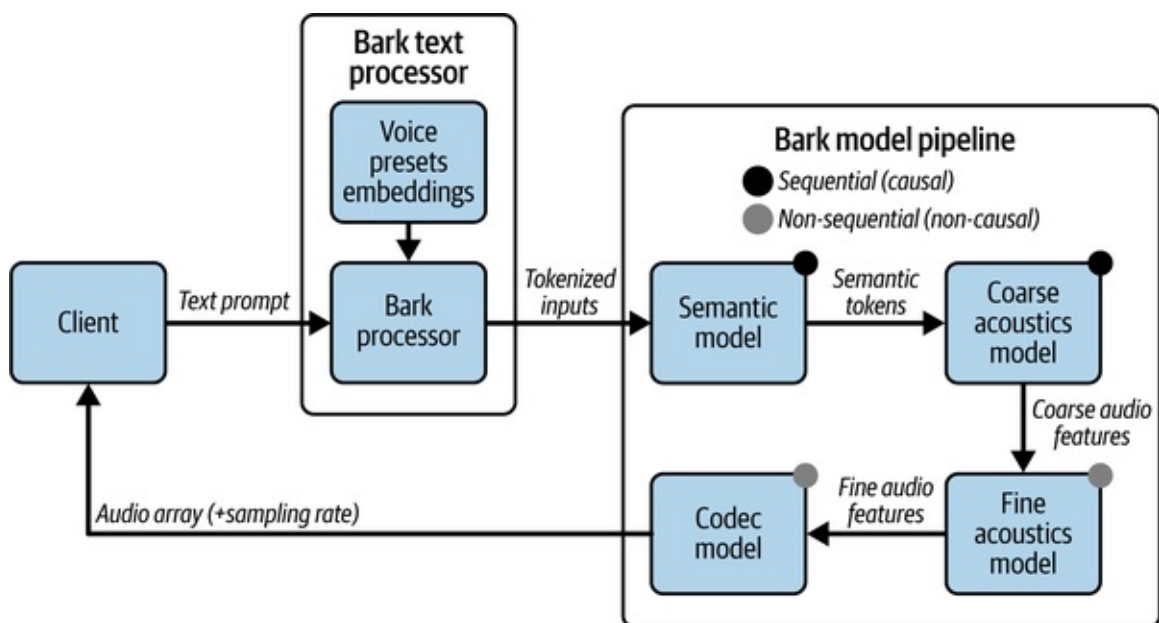
Figure 3-15. Bark synthesis pipeline
