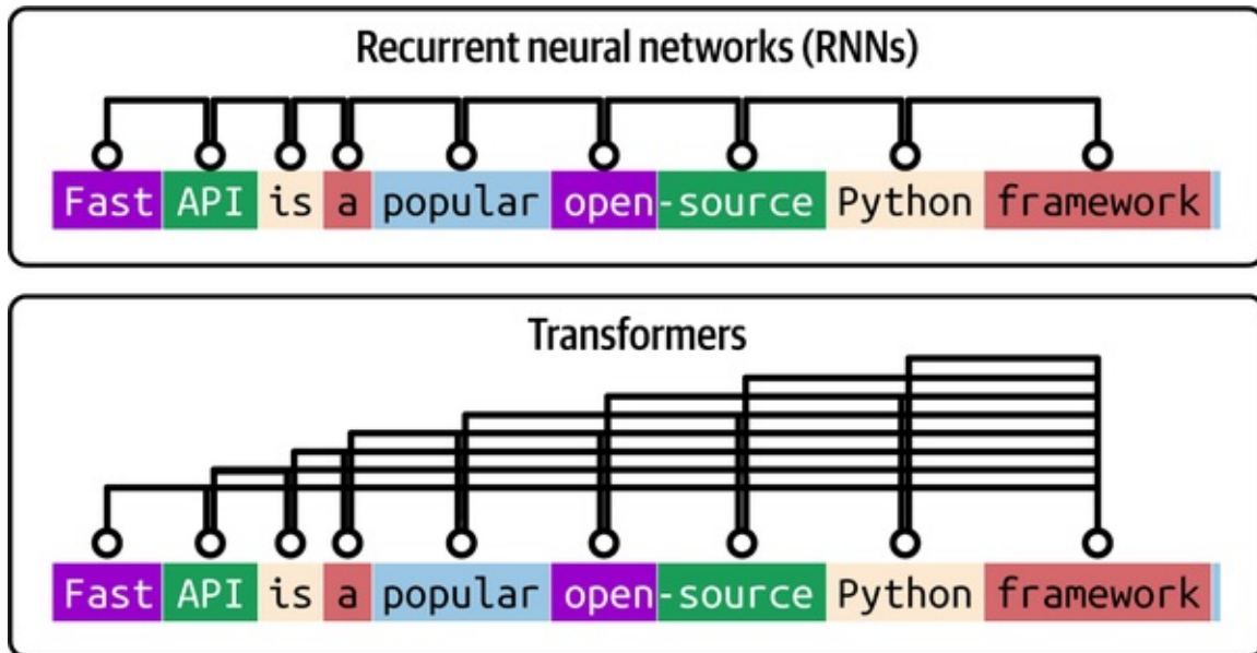
Figure 3-2. RNNs versus transformers in processing sentences
