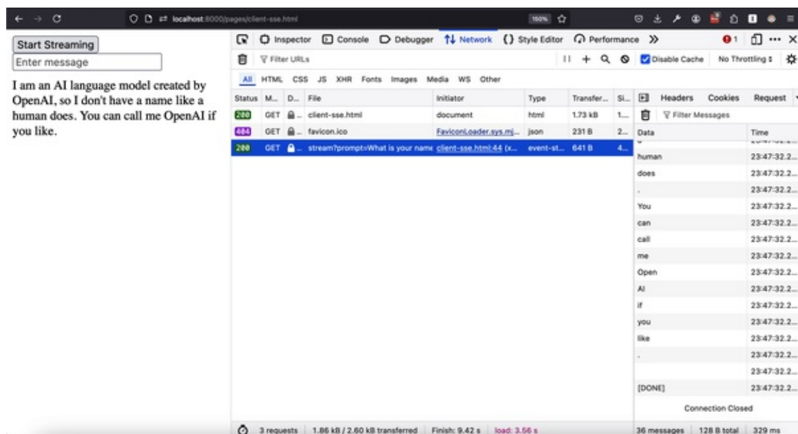
Figure 6-8. Incoming stream from the SSE endpoint
