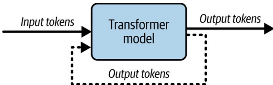
Figure 3-10. Autoregressive prediction
