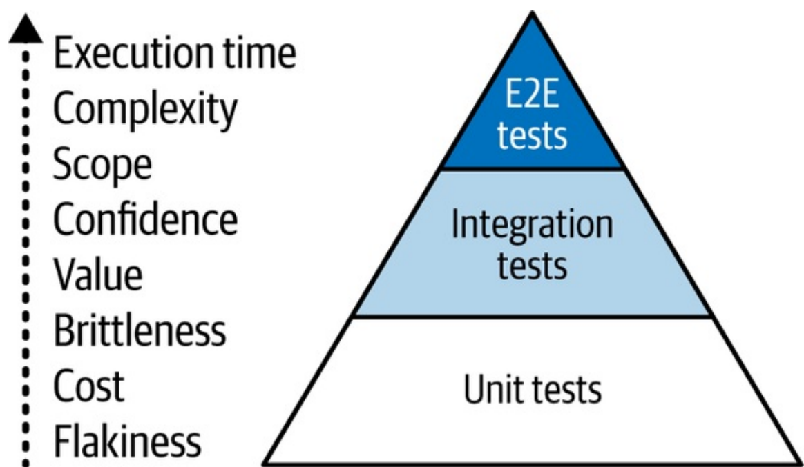
Figure 11-5. Testing pyramid
