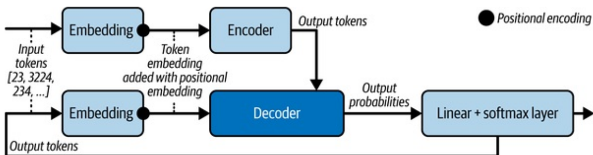
Figure 3-1. Transformer architecture
