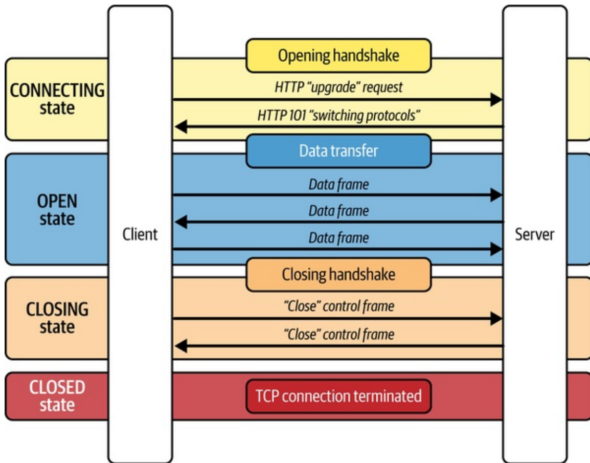
Figure 6-6. WebSocket connection lifecycle
