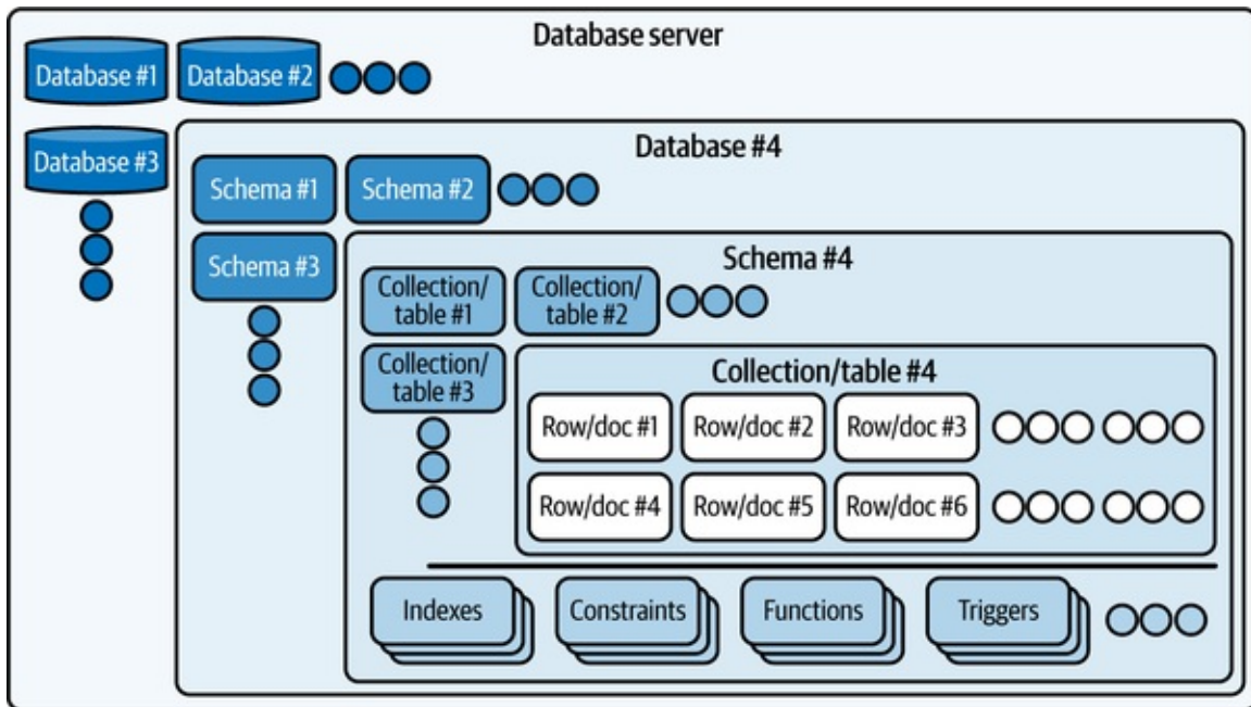
Figure 7-1. Database system breakdown
