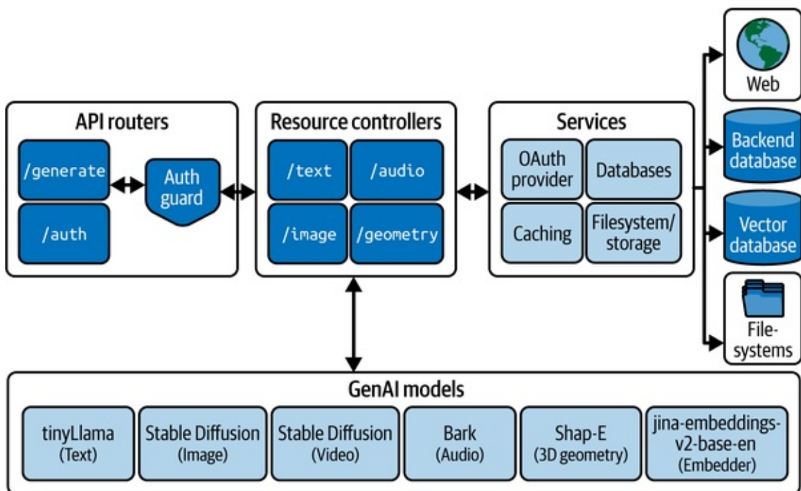
Figure 2-9. Generative AI service you'll build with FastAPI
