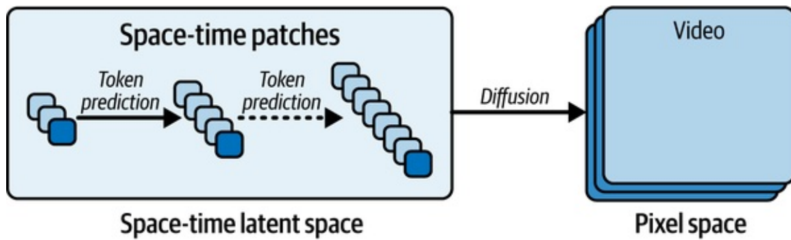
Figure 3-22. Token prediction by the vision transformer
