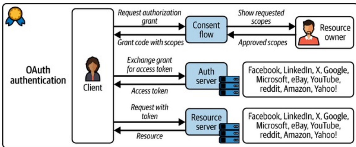
Figure 8-8. OAuth authentication flow
