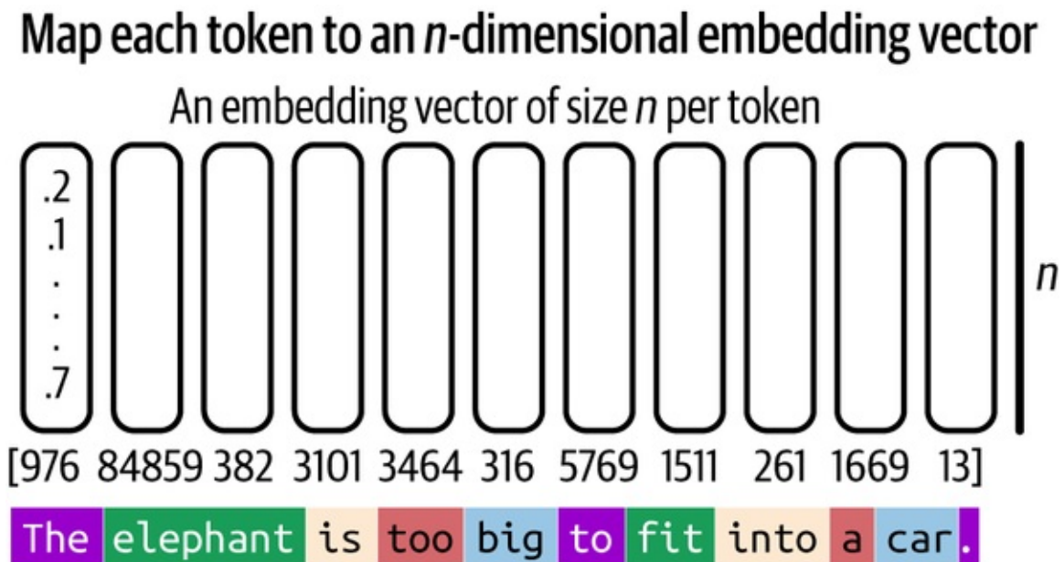
Figure 3-6. Assigning an embedding vector of size n to each token during the embedding process
