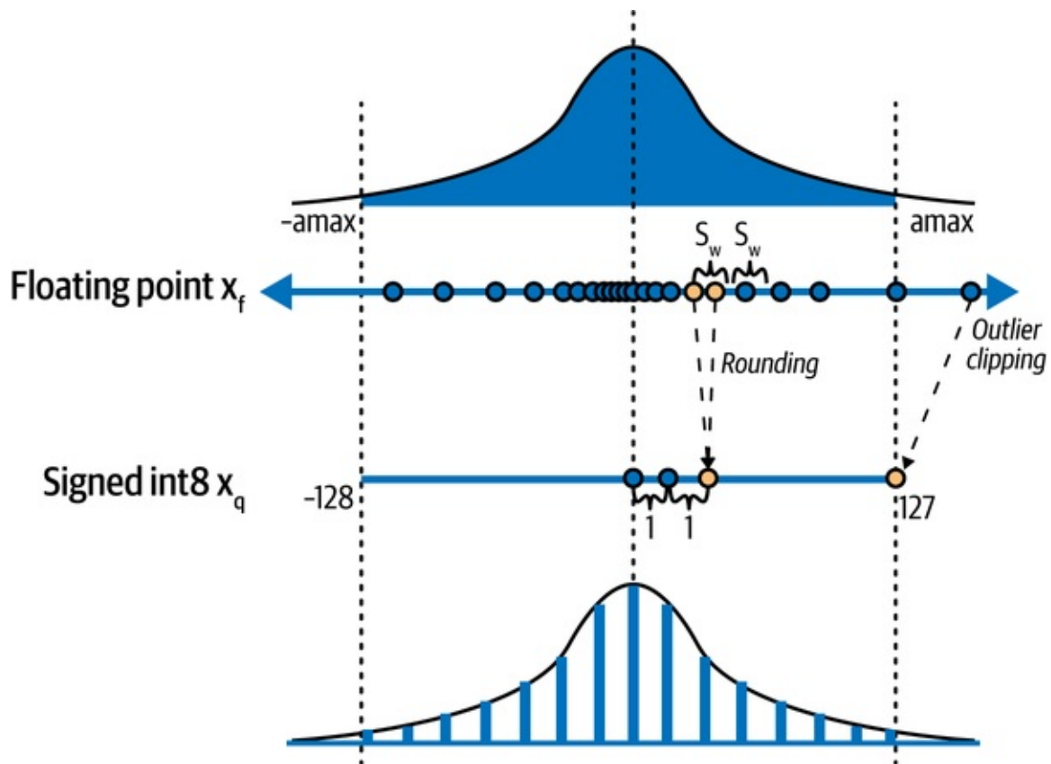
Figure 10-7. Quantization of floating-point numbers to integers
