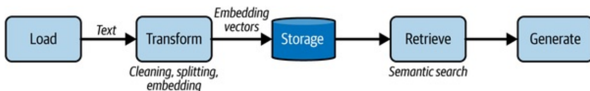
Figure 5-8. RAG pipeline
