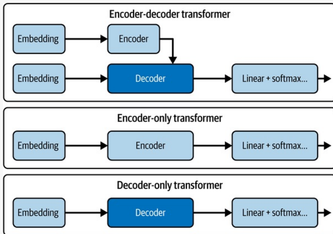
Figure 3-14. Transformer architectures
