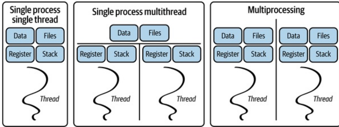
Figure 5-3. Resource sharing in multithreading and multiprocessing
