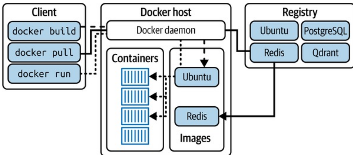
Figure 12-4. Docker platform system architecture
