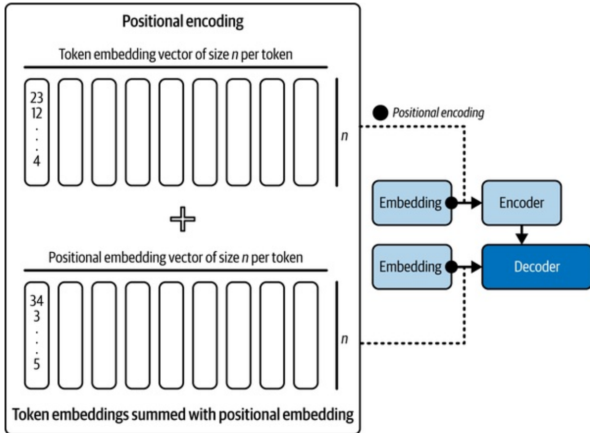
Figure 3-9. Positional encoding
