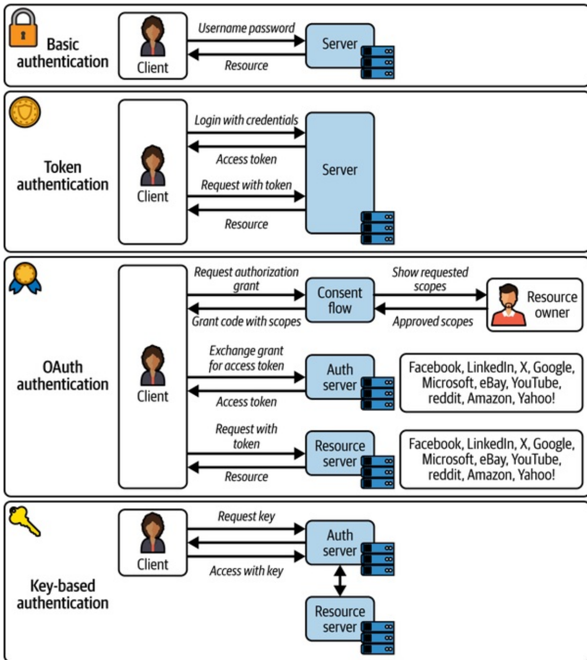
Figure 8-1. Authentication methods
