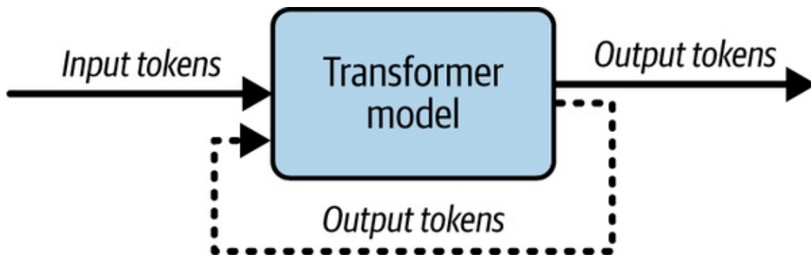
Figure 5-13. Autoregressive prediction
