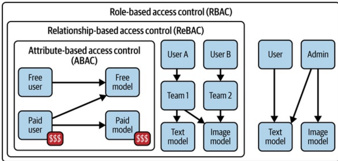
Figure 8-11. Authorization models
