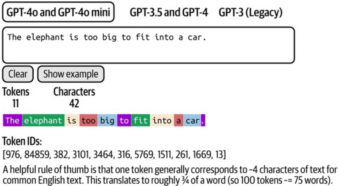
Figure 3-5. OpenAI tokenizer (Source: OpenAI )
