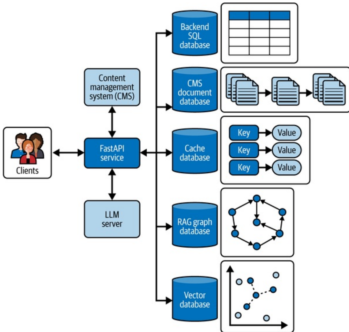
Figure 7-3. Using various database types together
