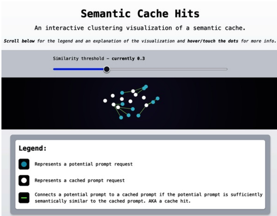
Figure 10-2. Visualization of semantic caching (Source: semanticcachehit.com )
