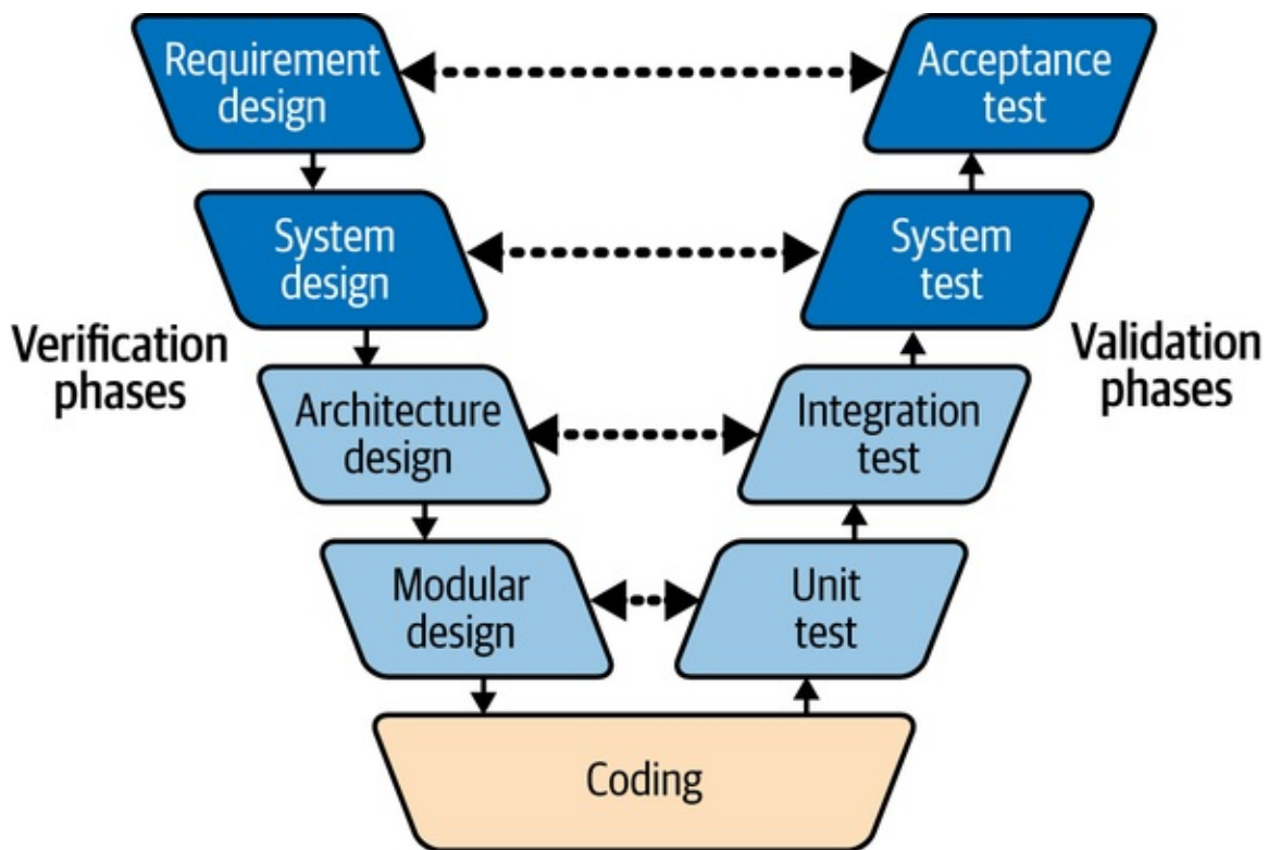
Figure 11-2. Verification and validation model
