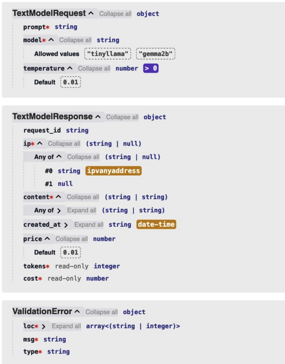
Figure 4-3. Automatic generation of FastAPI docs using Pydantic models
