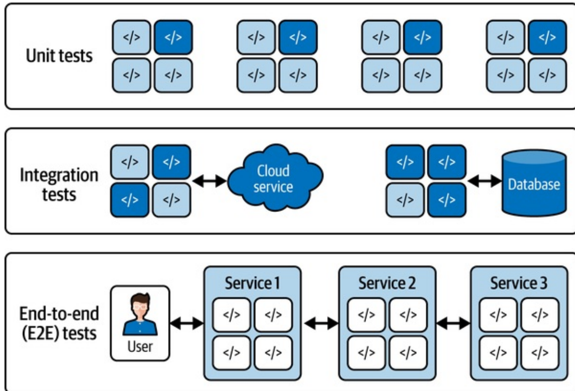
Figure 11-1. Types of tests in software testing
