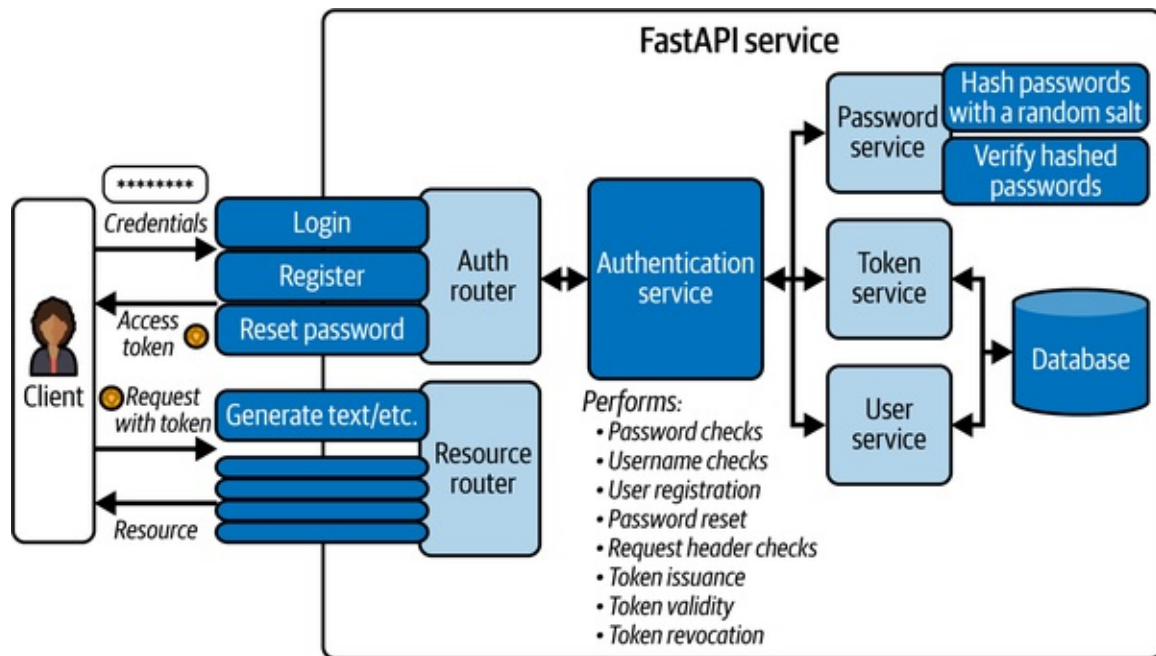
Figure 8-5. JWT authentication system architecture
