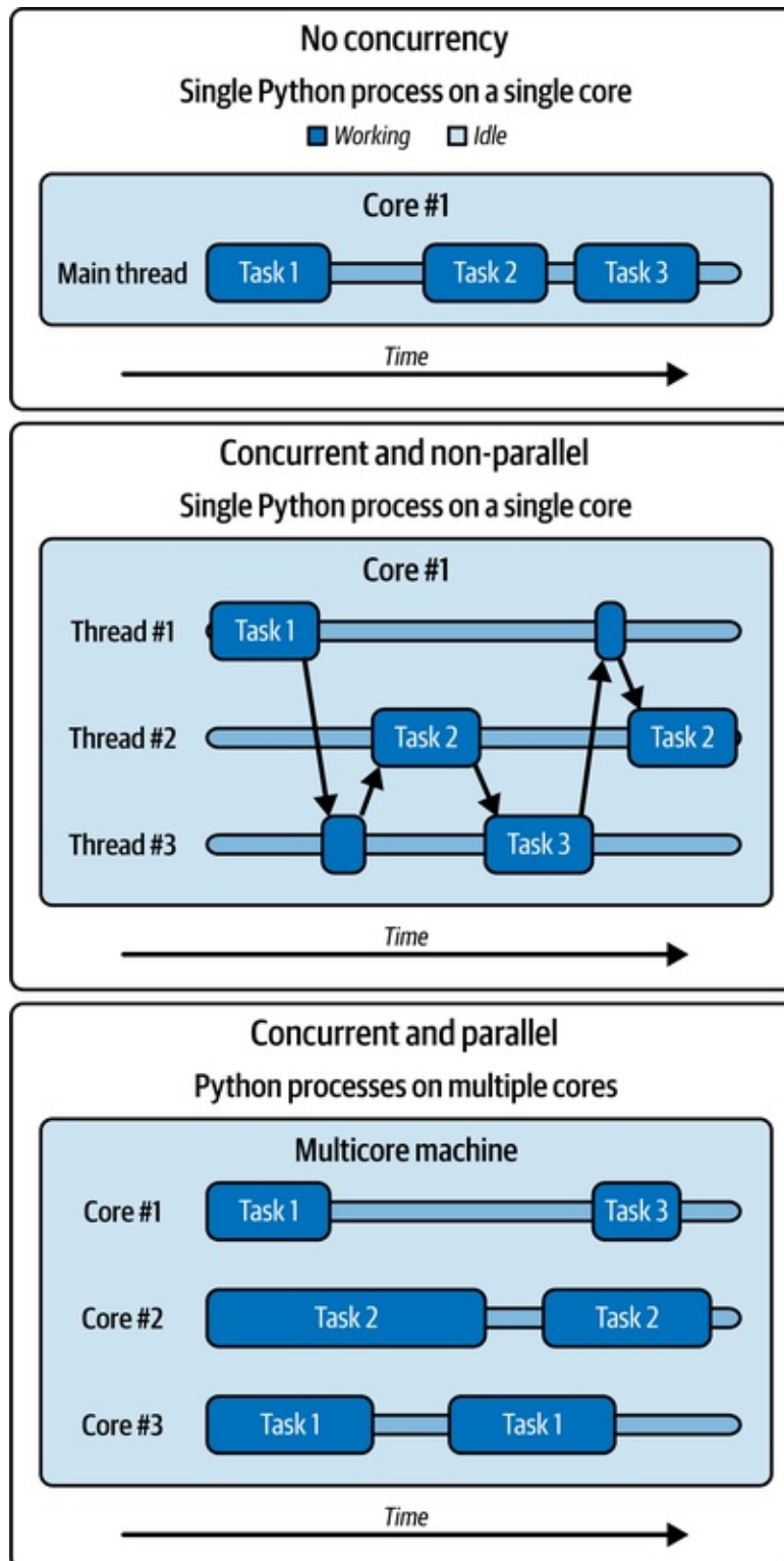
Figure 5-2. Concurrency with and without parallelism
