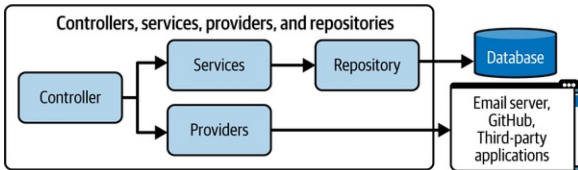
Figure 2-5. Services, providers, and repositories
