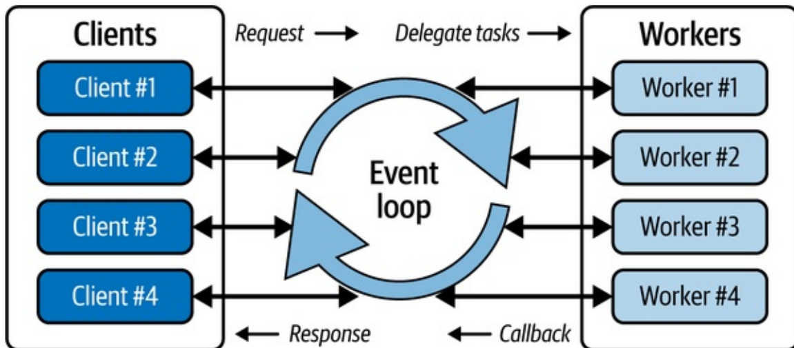
Figure 5-4. Async IO event loop
