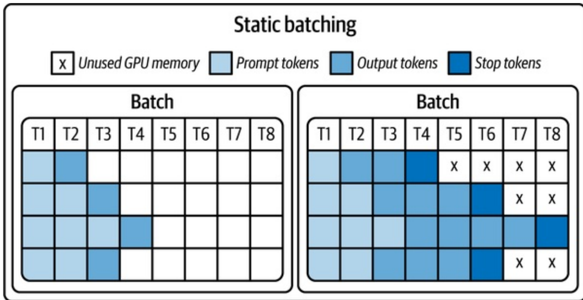
Figure 5-15. Static batching with fixed batch size
