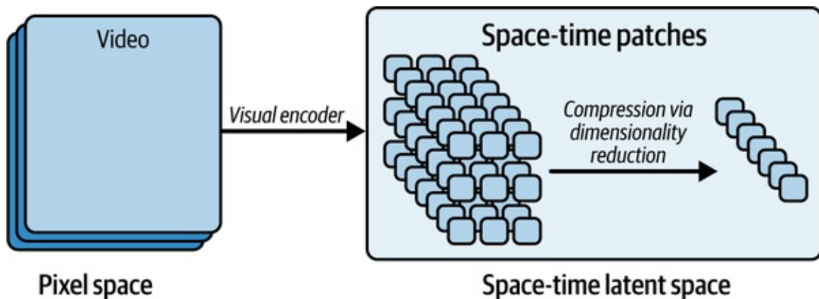
Figure 3-21. Video compression into space-time patches
