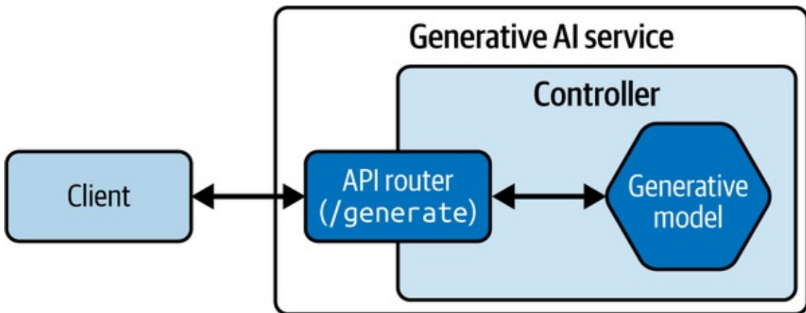
Figure 3-13. FastAPI service system architecture
