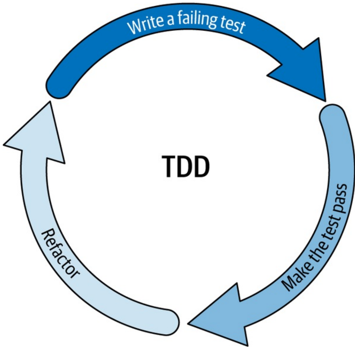
Figure 11-4. TDD
