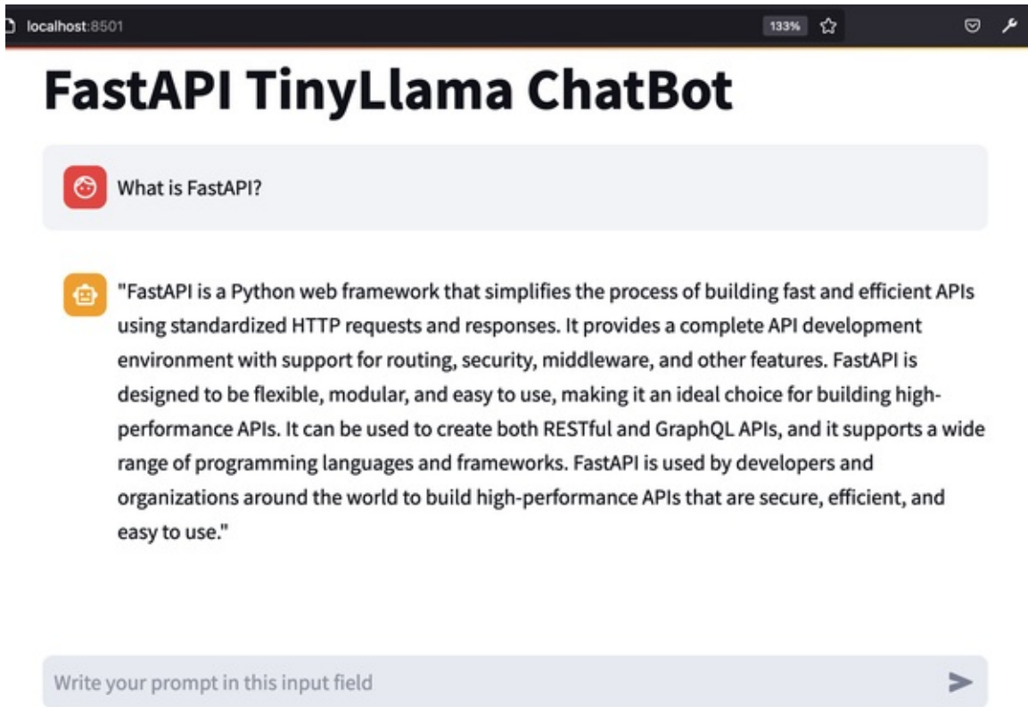
Figure 3-12. Streamlit client
