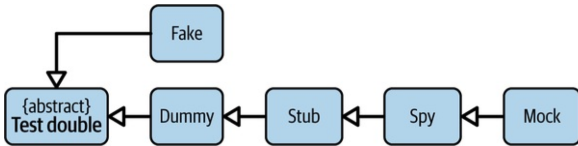
Figure 11-9. Test doubles
