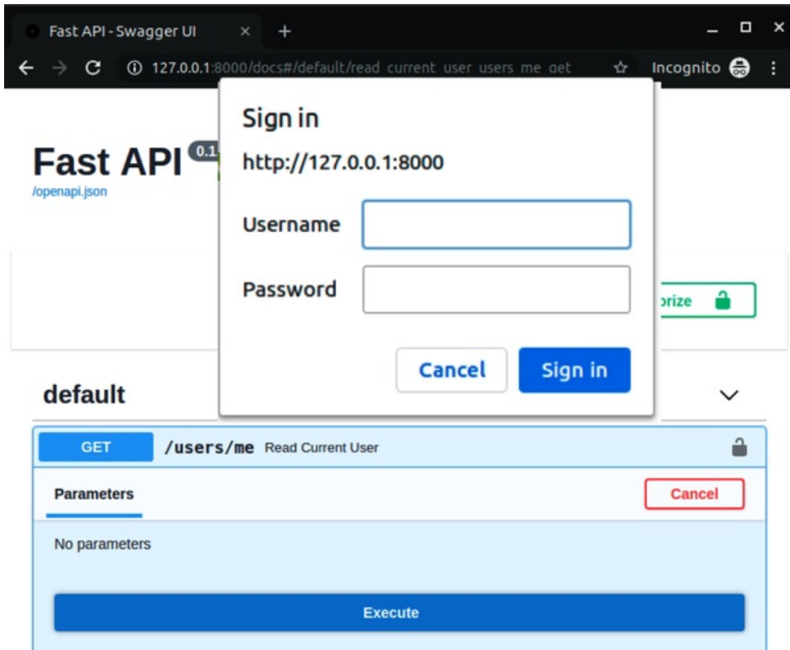
Figure 8-2. Basic authentication in FastAPI
